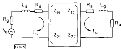
Fig. 5 Equivalent circuit of upconverter
