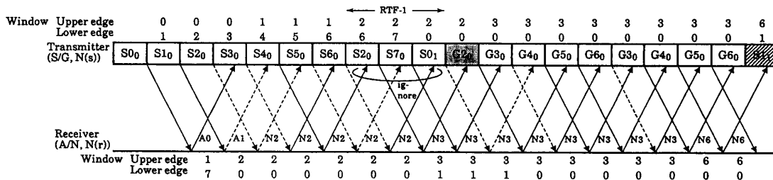
Fig.2 An example of WORM-ARQ operation
