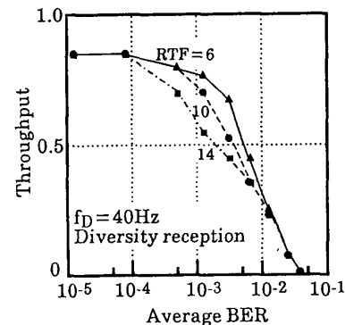
Fig.3 Throughput efficiency evaluated through computer simulations
