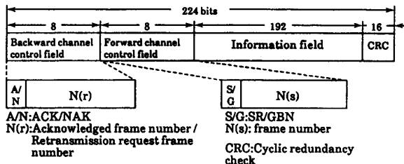
Fig.1 Frame format
