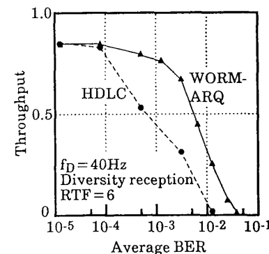
Fig.4 Throughput efficiencies with WORM-ARQ and HDLC evaluated through computer simulation
