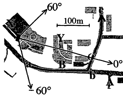
Figure 4. Measurement course for field tests
