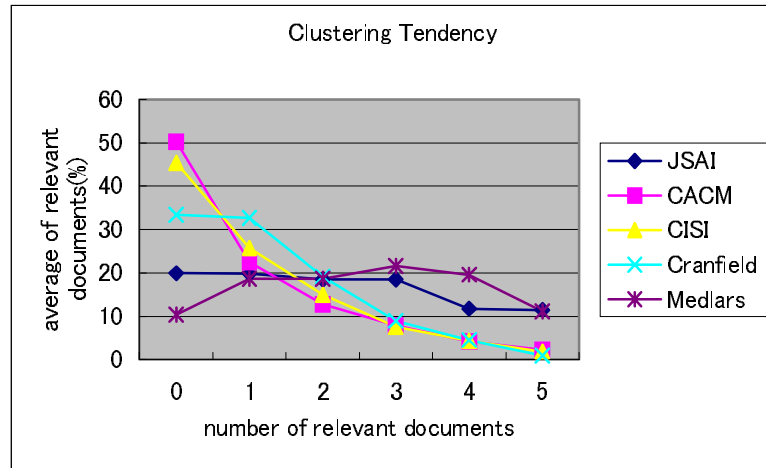
Figure 5-5: Clustering tendency
