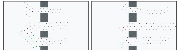
(a) t = 28[sec] (b) t = 40[sec] Fig. 12. Simulation results for flocking without the unification capability
