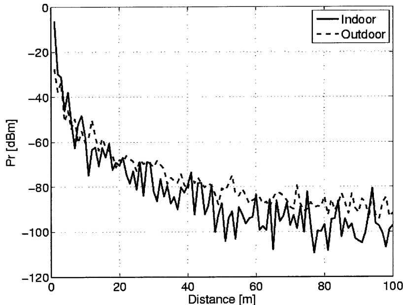
Figure 6: The received power, P_r , as function of the distance between the transmitter and the sender for indoor and outdoor environments (using parameter values from [Far-04]).
