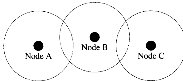
Figure 7: Example of the hidden node problem in a WLAN.
