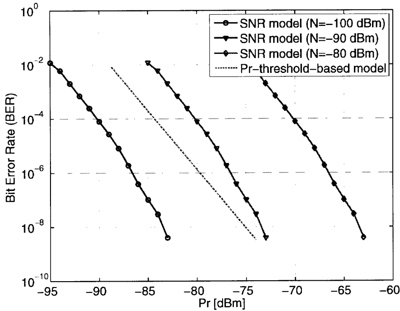
Figure 4: Bit error rate, BER, versus received power, P_r , according to the SNR model and several values of the noise power, N , as well as according to the P_r -threshold-based model for the 11 Mb/s operating rate.
