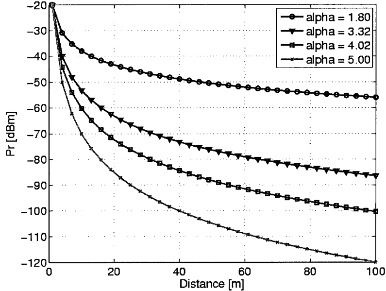
Figure 5: The received power, P_r , as function of the distance between the transmitter and the receiver for various values of \alpha ( \sigma = 0 dB).
