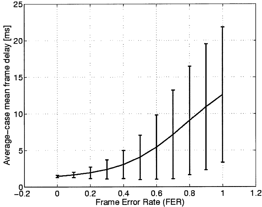
Figure 9: Average-case mean frame delay with jitter as error bars (11 Mb/s, 1024-byte-payload frames, r = 6 retransmissions).
