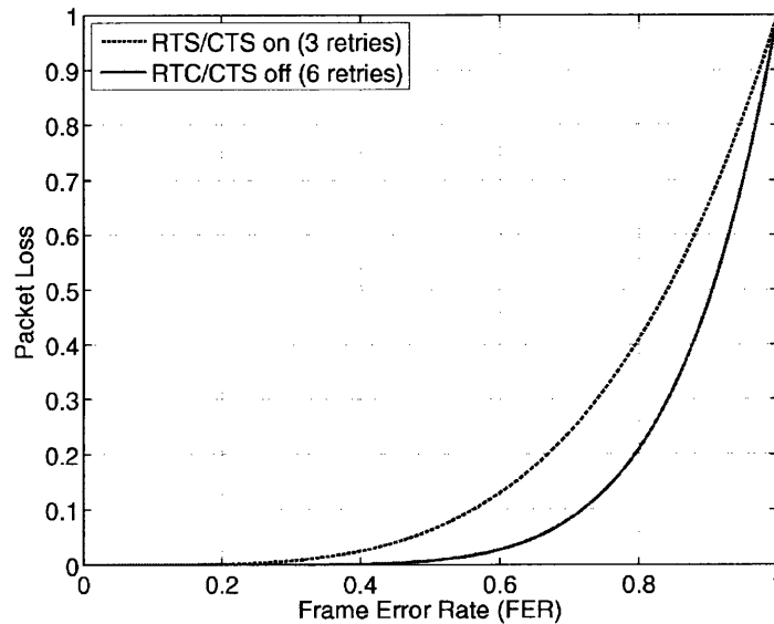
Figure 10: Packet loss versus frame error rate (considering the RTS/CTS protocol "on" or "off").
