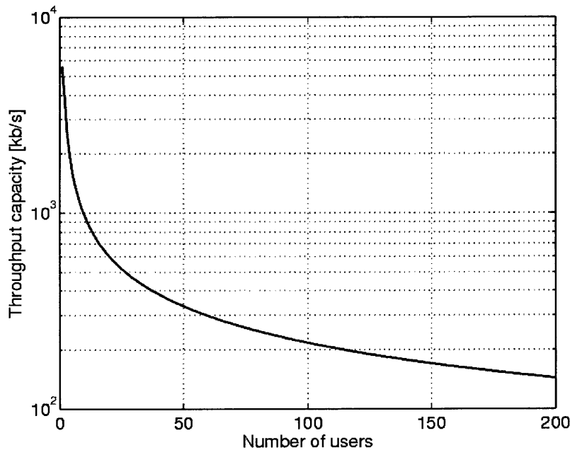
Figure 11: Throughput capacity in multi-user environments for the 11 Mb/s operating rate of 802.11.
