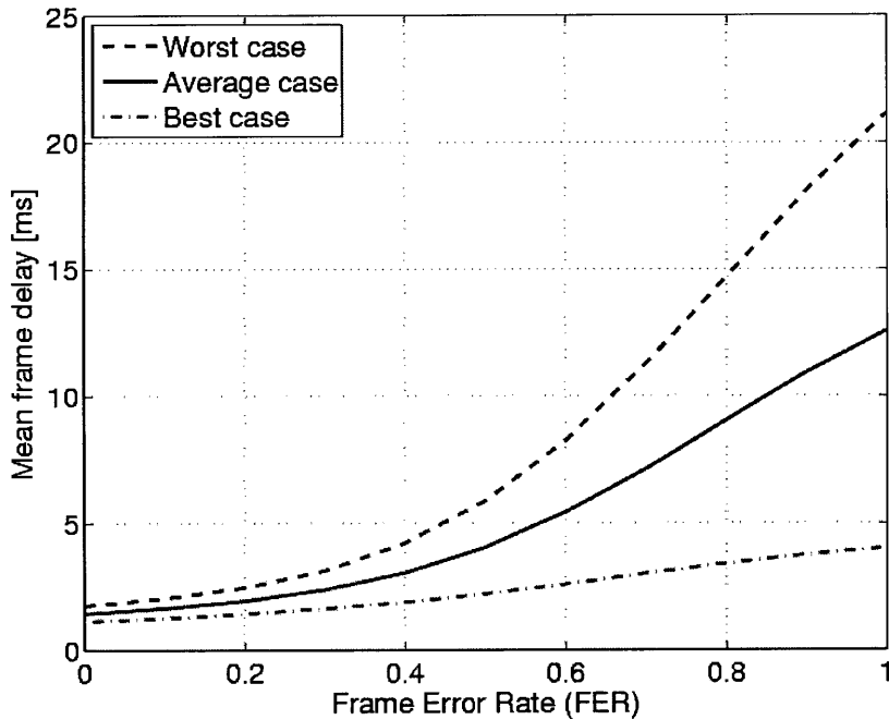
Figure 8: Mean frame delay for 11 Mb/s 1024-byte-payload frames versus frame error rate (number of retransmissions, r = 6 ) in the average, as well as best and worst cases.
