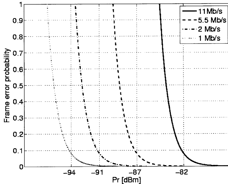
Figure 3: Frame error probability, FER_1 , versus received power, P_r , using an exponential-dependency model based on the P_r threshold and the associated frame error rate value.
