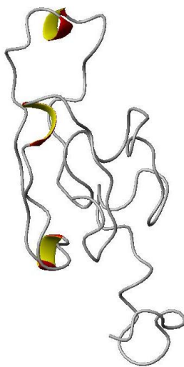
Fig.7. Conformation of 1j2m_min after 100ps MD simulation
