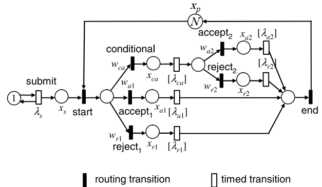
Fig. 6 RTCPN model.
