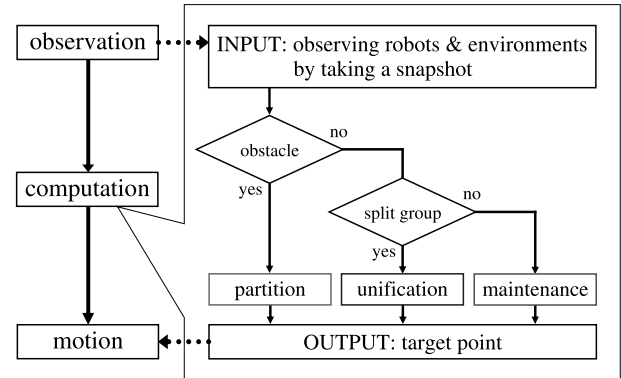
Fig. 2 Adaptive flocking flowchart.
