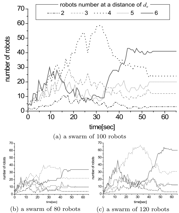
Fig. 8 Changes in the number of neighboring robots located at a constant distance of d_u from each robot in Fig. 7.
