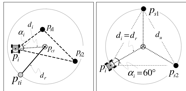
(a) two control parameters: range and bearing
