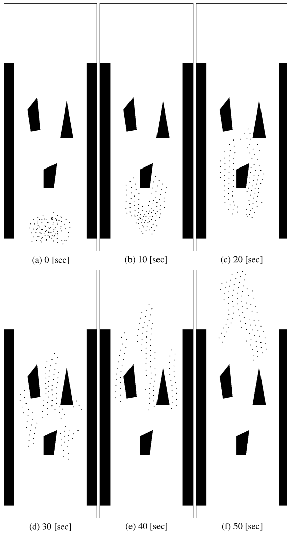
Fig. 7 Simulation results of adaptive flocking under static environmental conditions.
