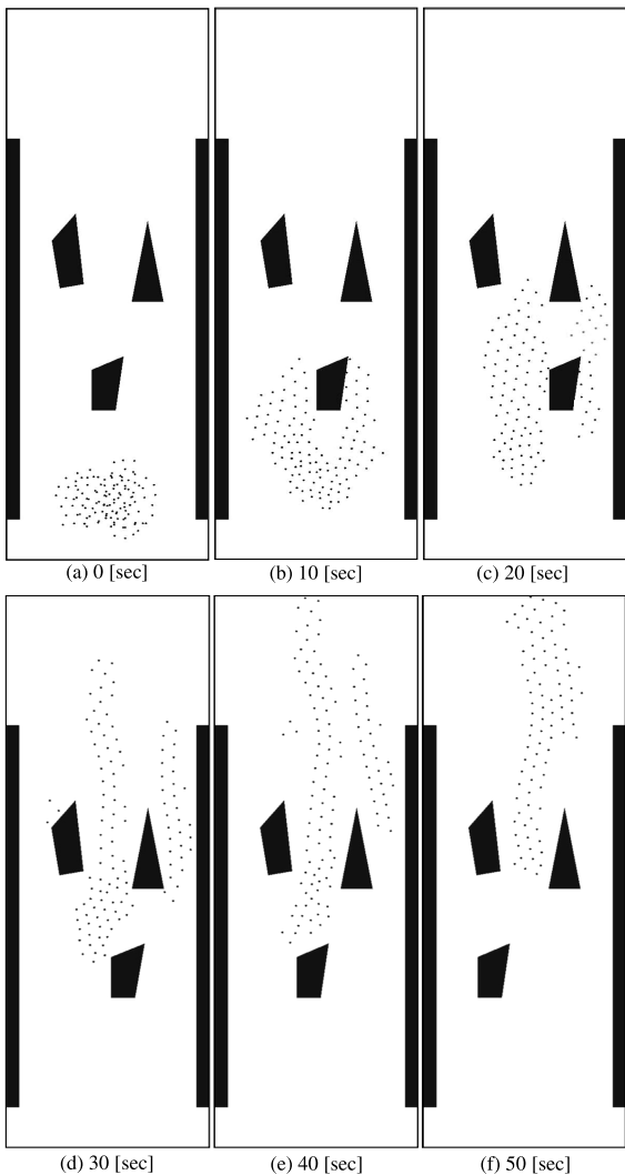
Fig. 9 Simulation results of adaptive flocking under dynamic environmental conditions.
