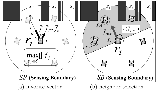
Fig. 5 Illustration of team partition.
