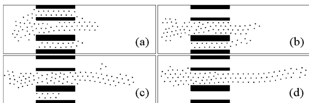
Fig. 10 Simulation results of adaptive flocking according to changes in sensing boundary (a) 2 times d_u , (b) 3.5 times d_u , (c) 6 times d_u , (d) 100 times d_u .
