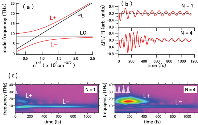
FIG. 2 (color). (a) L+ and L- modes (red) for g = 13 meV and bare plasmon and phonon (black). (b) Transient electro-optic responses \Delta R/R [\propto P_L(\tau) + P_E(\tau)] with r_L/r_E = 1 for the pulse train of N = 1 and N = 4 . (c) Continuous wavelet transformation of \Delta R/R in the frequency-time space. The density of doped carriers is n = 2 (\times 10^{18} \text{ cm}^{-3}) and the interval between pulses is \Delta = 2\pi/\omega_{L+} , i.e., 61 fs. The detuning \delta = 40 meV is adopted. The applied pulse train is illustrated.
