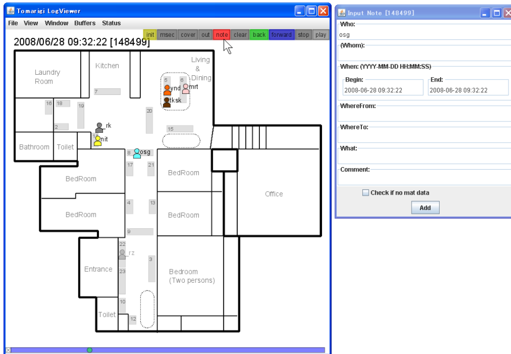
Figure 5. Logviewer (left) and annotation window (right).
