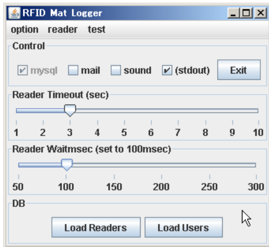
Figure 4. Event logger application.
