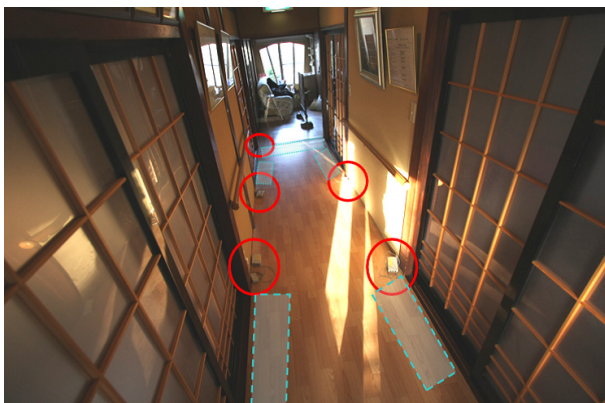
Figure 12. Deployment of an antenna in a corridor (before mounting RFID reader boxes).
