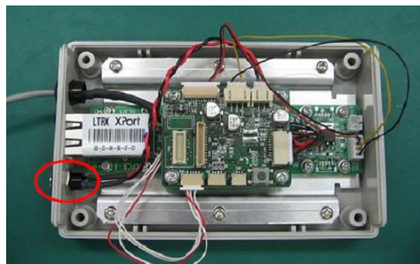
Figure 2. RFID reader box.
