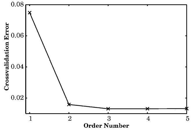
FIG. 1. Cross-validation test applied to coupled limit cycle predator-prey model. For order number \mu=1,2,\dots,5 , error function E_c is computed for the test data, which are not used for the parameter estimation. The minimum error points the optimum Fourier order at \mu=3 .
