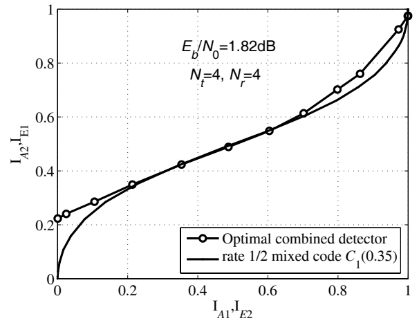
Fig. 4. EXIT charts of the optimal combined detector with N_t = N_r = 4 at E_b/N_0=1.82\text{dB} and a rate-1/2 mixed code C_1(0.35) , which is a mixture of rate-1/2 4-state and 2-state codes with code doping ratio \alpha = 0.35 .
