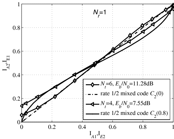
Fig. 6. EXIT curves of the optimal combined detector with ( N_t=6 , N_r=1 ) and ( N_t=4 , N_r=1 ) antennas at E_b/N_0=11.28 dB and E_b/N_0=7.55 dB, respectively, and EXIT curves of rate-1/2 mixed codes C_2(0) and C_2(0.8) .
