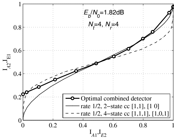
Fig. 3. EXIT charts of the optimal combined detector with N_t = N_r = 4 at E_b/N_0=1.82\text{dB} , rate-1/2, 2-state cc with \mathbf{g}_1 = [1, 1] and \mathbf{g}_2 = [1, 0] , and rate-1/2 4-state cc with \mathbf{g}_1 = [1, 1, 1] and \mathbf{g}_2 = [1, 0, 1] .
