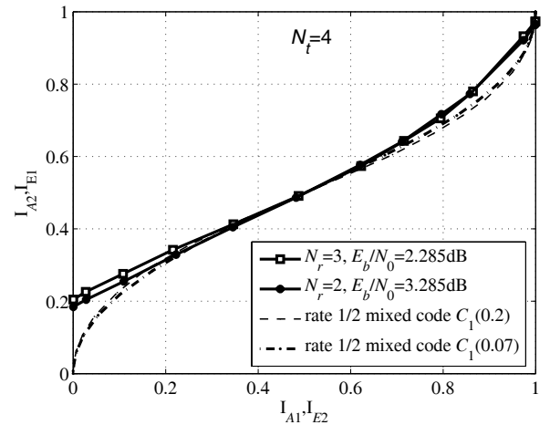
Fig. 5. EXIT charts of the optimal combined detector in various asymmetric scenarios using N_t = 4 and N_r = 3 at E_b/N_0=2.285\text{dB} , N_t = 4 and N_r = 2 at E_b/N_0=3.285\text{dB} , and rate-1/2, mixed codes C_1(0.2) and C_1(0.07) .
