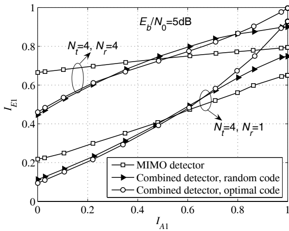
Fig. 2. The MIMO and combined detector EXIT curves at E_b/N_0=5\text{dB} .
