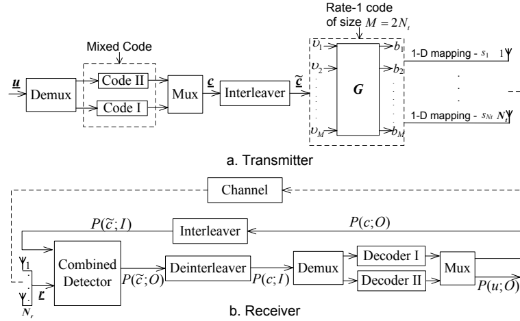
Fig. 1. The proposed concatenation scheme equipped with N_t transmit and N_r receive antennas.
