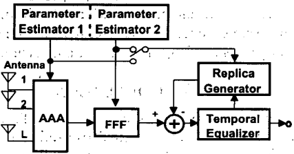
Fig. 2: Proposed S/T-Equalizer
