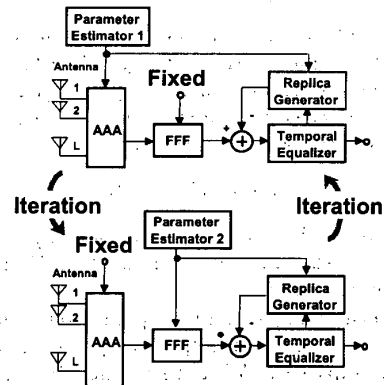
Fig. 4: Proposed Iterative S/T-Equalizer
