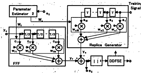
(b) Signal Processing of PE-2
