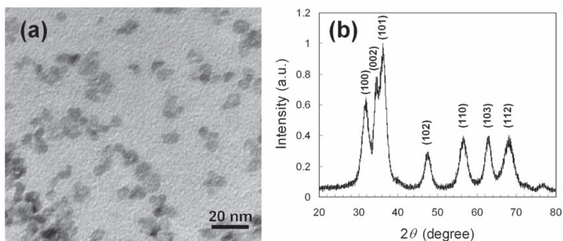
Fig. 1. (a) Transmission electron microscope image of as-synthesized ZnO NPs with a mean diameter 5.4 nm. (b) XRD pattern of ZnO NPs indicating that their crystal structure is wurtzite.
