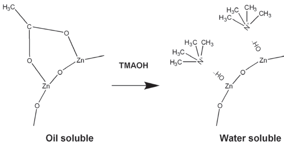
Fig. 2. Schematic illustration of ligand exchange
