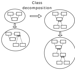
Figure 5.3: Agent decomposition
