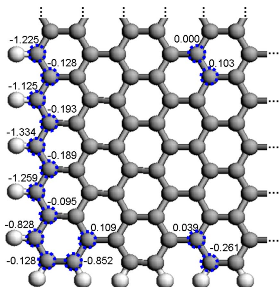
FIG. 5. (Color online) Position dependence of stability of doped N. The total energy for an N atom sitting nearly at the center of the cluster is taken as the reference. The relative total energy in eV for different site of doped N is listed. The results show that the doped N favors the zigzag edge sites.
