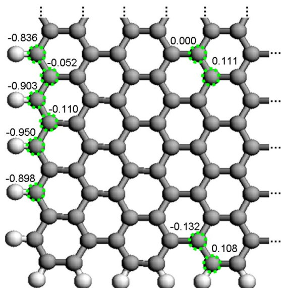
FIG. 12. (Color online) Position dependence of stability of doped B. The total energy for a B atom sitting nearly at the center of the cluster is taken as the reference. The relative total energy in eV for different site of doped B is listed. The results show that the doped B also favors the zigzag edge sites.
