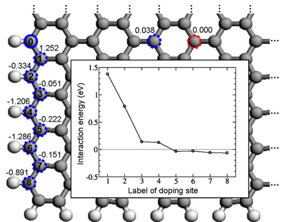
FIG. 11. (Color online) Graphene cluster with two N dopants. One of the two N dopants is always located at the site numbered “0” along the zigzag edge. The total energy of the system with two N dopants is measured with reference to the case where the second N dopant is located at the center of the cluster. The number shown at each site denotes the relative total energy (in eV) of the system where the second N dopant is located at the site. The inset plot denotes the interaction energy (in eV) between two N dopants, the first one being at the site labeled as 0 and the second one at another site.
