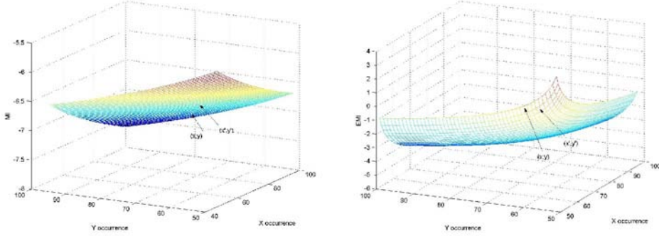
Figure 3 Plots of MI (left) and EMI (right) for association measure of (x, y) and (x', y') , respectively. Their co-occurrence is fixed as 50 and occurrences of two words are varying in their axes.
