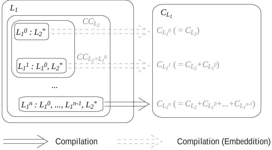
Figure A.3: A way of implementation by embedding meta-codes
