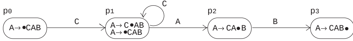
Figure 4.3: Mono for G_4
