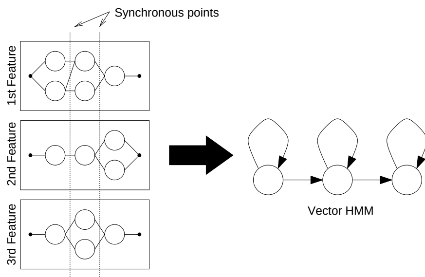
(A) Synchronous FD-SSS
