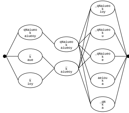
9th MFCC
