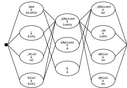
8th MFCC
