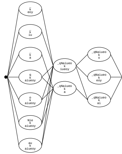
6th MFCC
