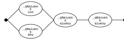
12th MFCC
