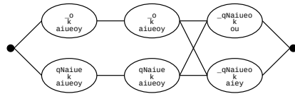
11th MFCC
