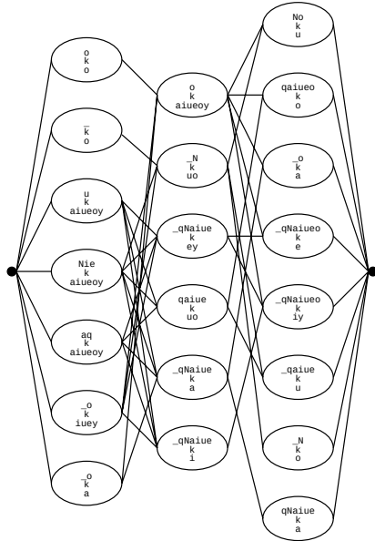
3rd MFCC
