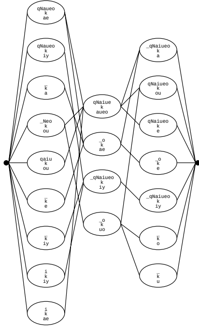
1st MFCC
