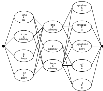
7th MFCC
