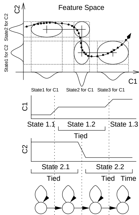
(B) Modeling by the temporal tying technique
