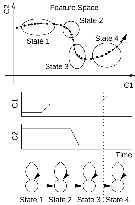
(A) Modeling by conventional HMM
