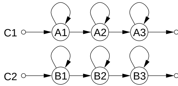
(1) Non-sequenced AT-HMM implemented using scalar HMMs.
