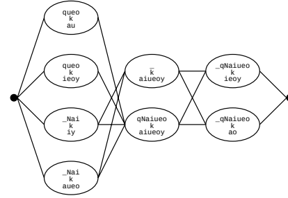
10th MFCC
