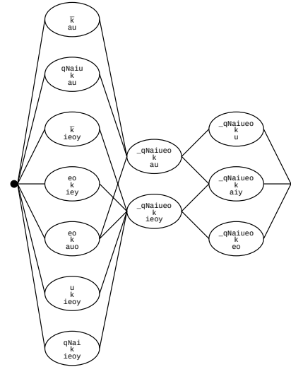
4th MFCC
