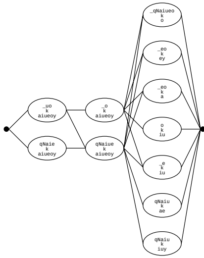
5th MFCC
