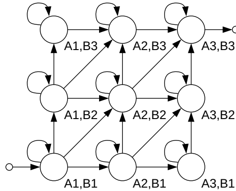
(2) Non-sequenced AT-HMM implemented using direct-product HMM.
