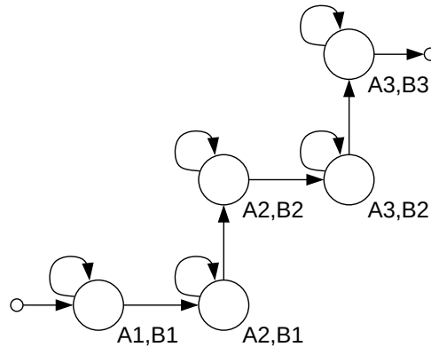
(3) Sequenced AT-HMM implemented using direct-product HMM.
