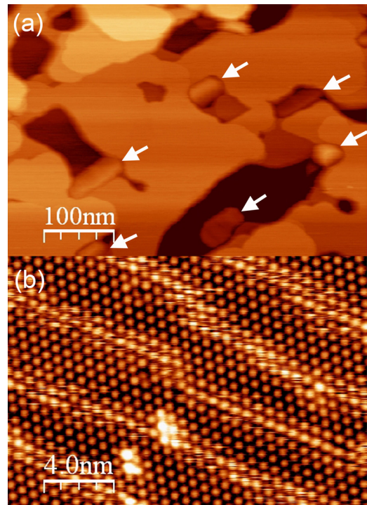
FIG. 2. (Color online) STM images observed for a \text{ZrB}_2 thin film surface after oxide removal. (a) A large-scale image observed with sample bias voltage ( V_s ) of +1 V, and tunneling current ( I ) of 32 pA. White arrows indicate protrusions which are \text{ZrB}_2 crystallites misoriented from the dominant \text{ZrB}_2(0001)\parallel\text{Si}(111) relation. (b) A high-resolution \text{ZrB}_2(0001) - (2 \times 2) image observed at an atomically-flat region with V_s = -0.3 V and I = 61 pA. Domain boundaries show a brighter contrast.
