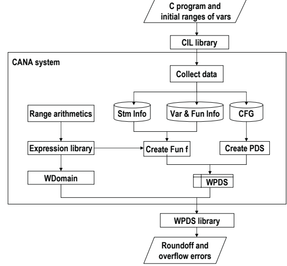
Figure 4. CANA system
