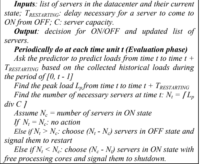
Figure 6. Pseudo-code of the algorithm.
