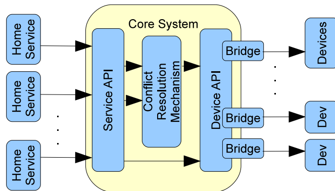
Figure 4.1: System Overview
