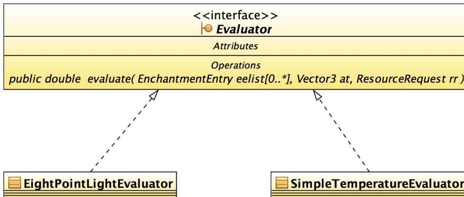
Figure 4.13: Evaluators
