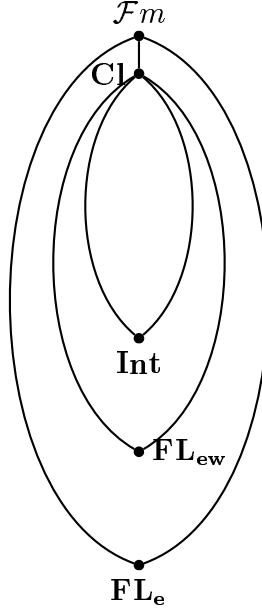
Figure 2.1: the lattice of \mathbf{CSL}
