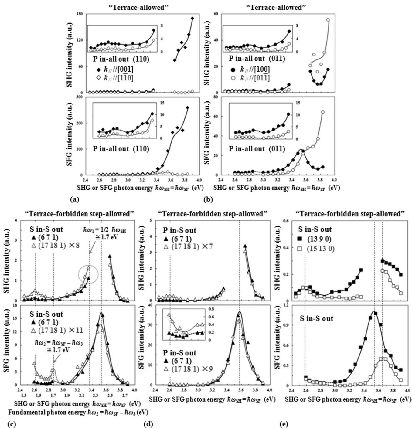
FIG. 8. SHG and SFG spectra of (a) TiO 2 (110) at P in-all out, (b) TiO 2 (011) at P in-all out, (c) TiO 2 (671) and (17181) at S in-S out, (d) TiO 2 (671) and (17181) at P in-S out, and (e) TiO 2 (1390) and (15130) at S in-S out. Incident angles of fundamental beams were set to \sim 45^\circ for (a) and (b), and were set to \sim 2^\circ for (c), (d), and (e). Directions of the incident planes are shown in Fig. 3.
