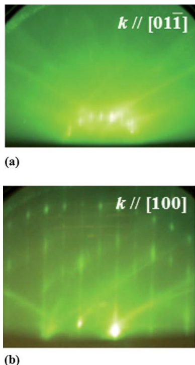
FIG. 6. RHEED patterns of TiO 2 (011). k vectors of electron beams were set parallel to (a) [0\bar{1}\bar{1}] and (b) [100] .
