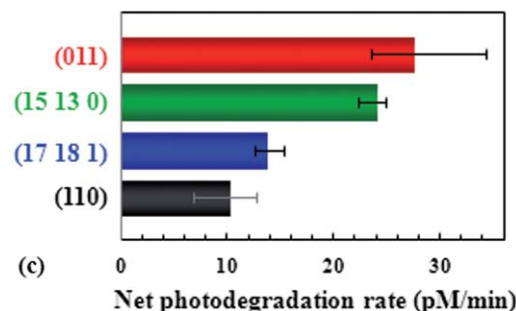
FIG. 7. (a) Transmission spectra of a methylene blue aqueous solution before and after three-hour UV illumination on TiO 2 (011). (b) Changes in the concentration of methylene blue molecules as a function of UV irradiation time for each sample. Each data set was fitted with an exponential decay curve to estimate a photodegradation rate. (c) Net photodegradation rates were estimated through the exponential fitting in (b).
