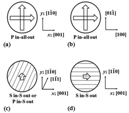
FIG. 3. Directions of incident beams (incident planes) in the SHG/SFG spectroscopy for (a) \text{TiO}_2 (110), (b) \text{TiO}_2 (011), (c) \text{TiO}_2 (6 7 1) and (17 18 1), and (d) \text{TiO}_2 (13 9 0) and (15 13 0). The arrows represent parallel components of incident wave vectors to a surface, \vec{k}_{//} . Step edges on the \text{TiO}_2 vicinal surfaces are indicated by solid lines.
