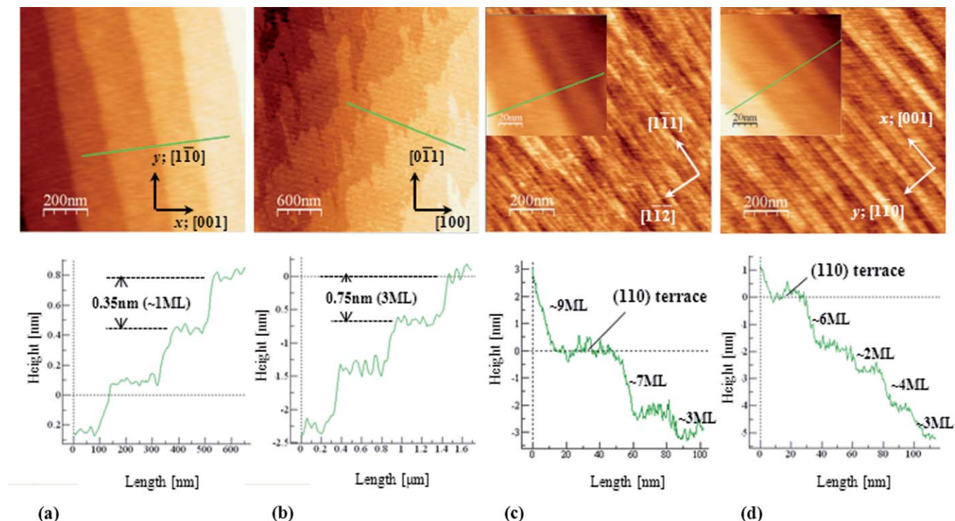
FIG. 4. Contact AFM images and their height profiles of (a) TiO 2 (110) (scanning area: 1.0 \times 1.0 \mu\text{m}^2 ), (b) TiO 2 (011) ( 3.0 \times 3.0 \mu\text{m}^2 ), (c) TiO 2 (17 18 1) ( 1.0 \times 1.0 \mu\text{m}^2 ), and (d) TiO 2 (15 13 0) ( 1.0 \times 1.0 \mu\text{m}^2 ). Scanning areas of the insets in the images (c) and (d) are 100 \times 100 \text{ nm}^2 .
