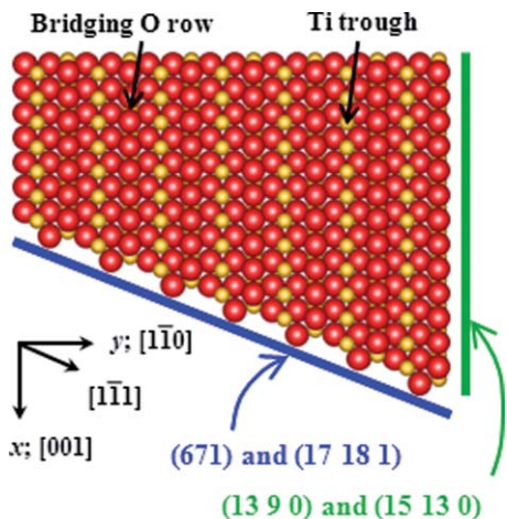
FIG. 5. Expected top edge structures of the step bunches corresponding to the (6 7 1), (17 18 1), (13 9 0), and (15 13 0) vicinal surfaces.
