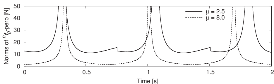
Fig. 5. Time evolution of norms of {}^p f_g^\perp for \mu = 2.5 and 8.0 in VPDW with CTR formula.
