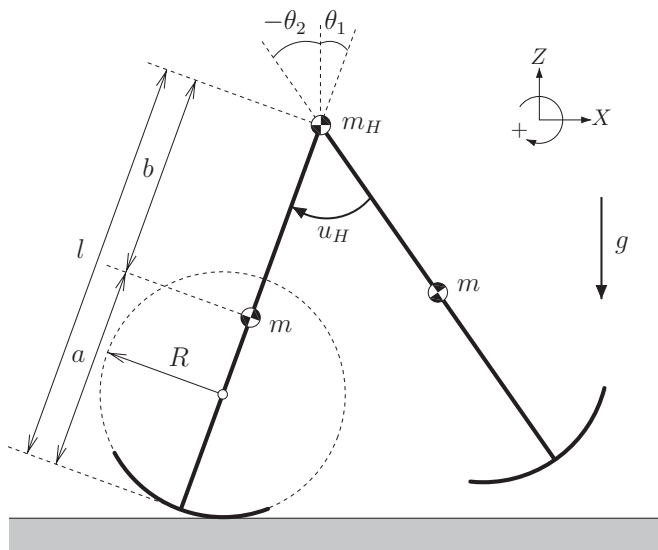
Fig. 7. Model of planar underactuated biped robot with semicircular feet.
