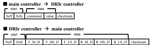
(c) two kinds of communication packets
