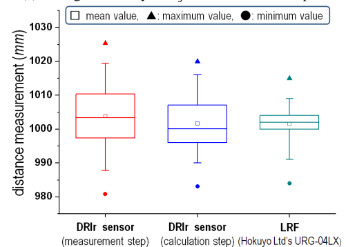
(d) comparison between DRIR sensor and LRF
