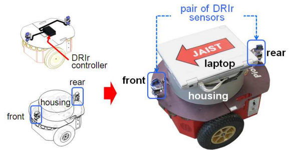
(a) mobile robot integration
