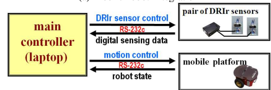
(b) overall control schematic
