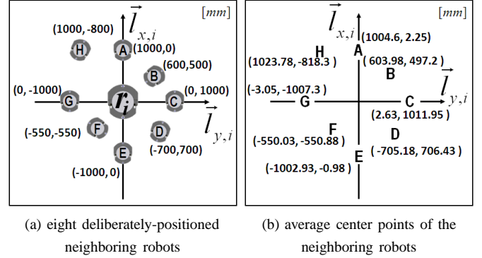
Fig. 14. Observation results for deliberately positioned 8 neighboring robots
