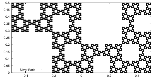
Figure 7: The set of the first 10000 points given by the silver ratio \phi = \sqrt{2} - 1 = \frac{1}{2+\frac{1}{2+\frac{1}{2+\dots}}} .
